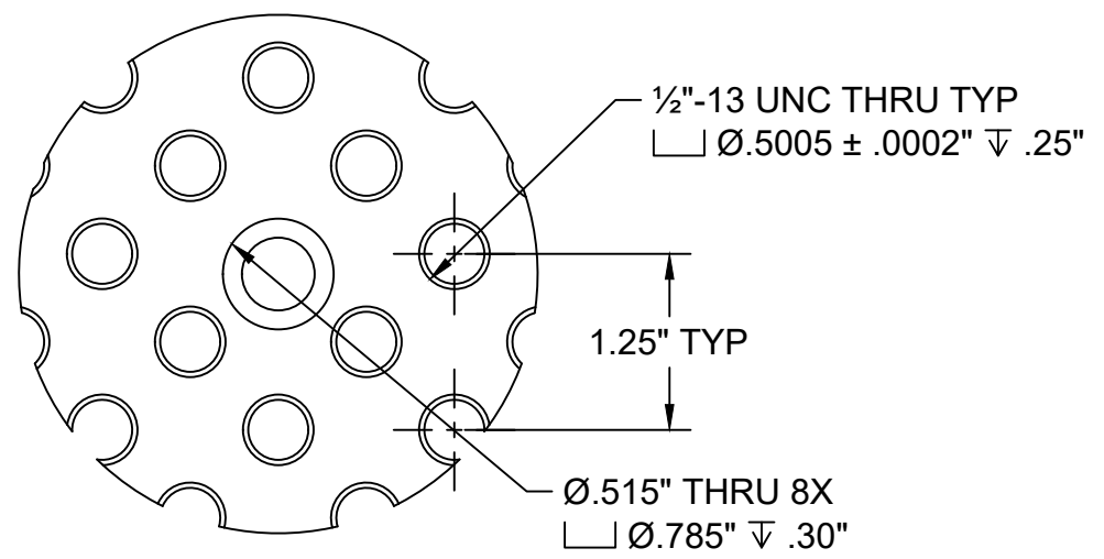
DETAIL A SCALE 2:3
