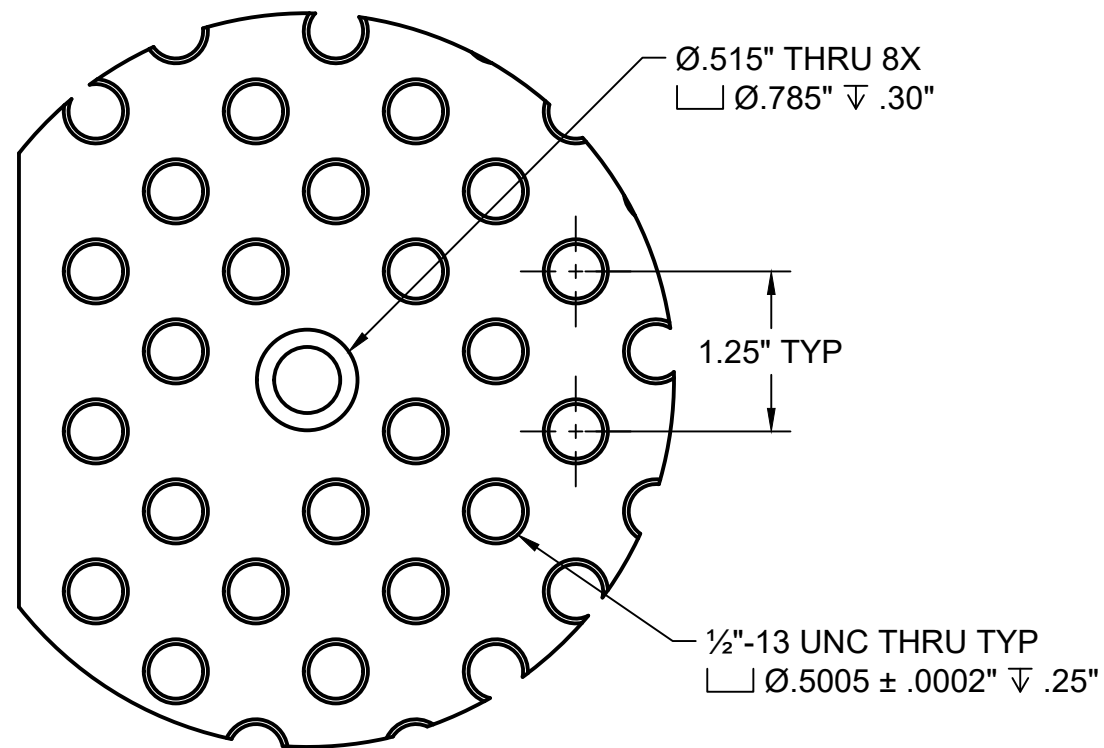
DETAIL A SCALE 2:3
